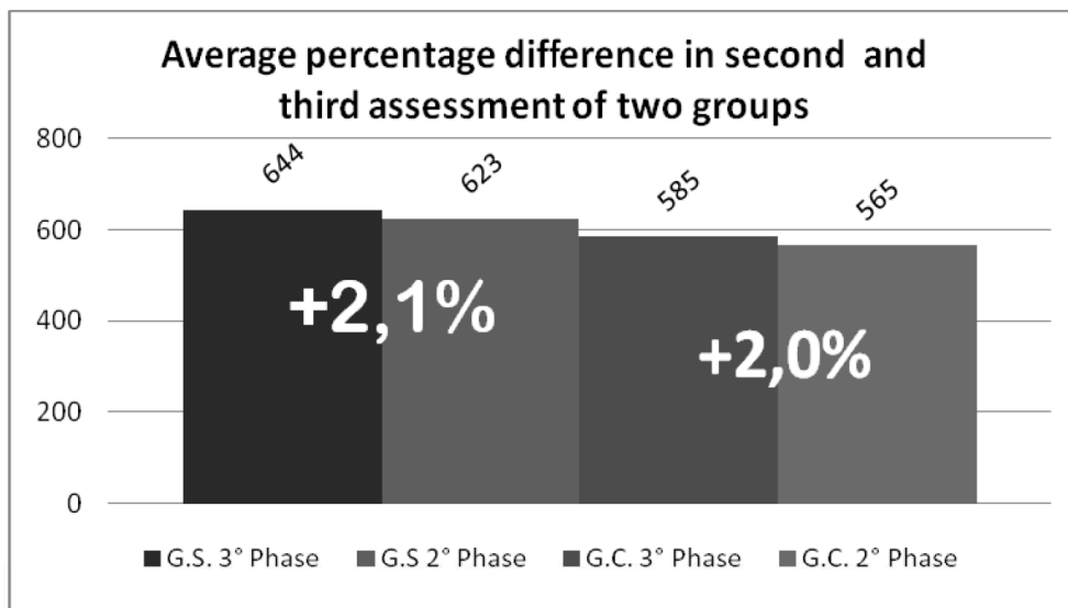
Fig. 3 : Comparison of the difference of average percentage scores in second and third assessment of two groups
