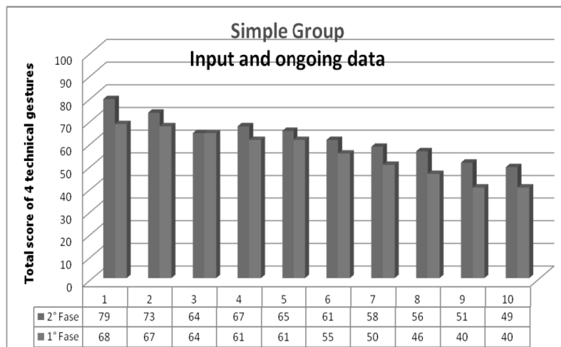
Fig.2: (2nd phase) Comparison of the assessments in the sample group of observations in input and ongoing with an average improvement of +7.1%
