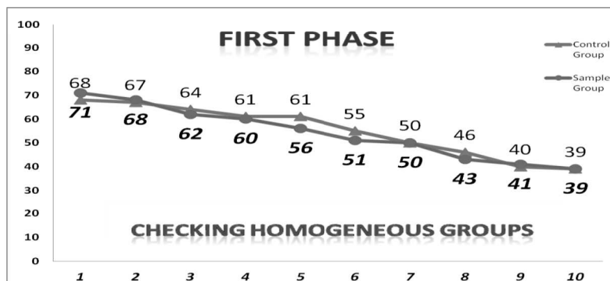
Fig. 1: (1 th Phase ) Evaluation grid of the technician: data in input phase of Simple Group and Contol Group
