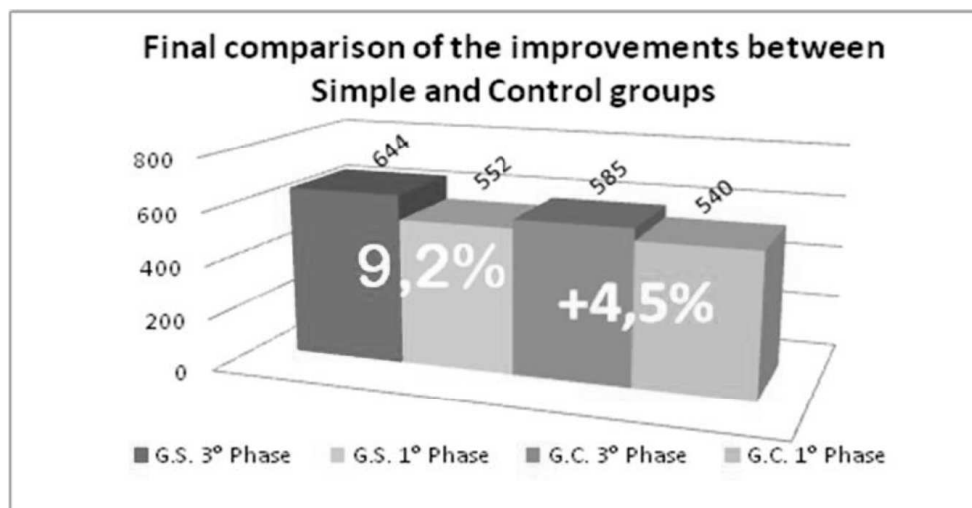
Fig. 4 : Final comparison of the improvements between Simple and Control groups
