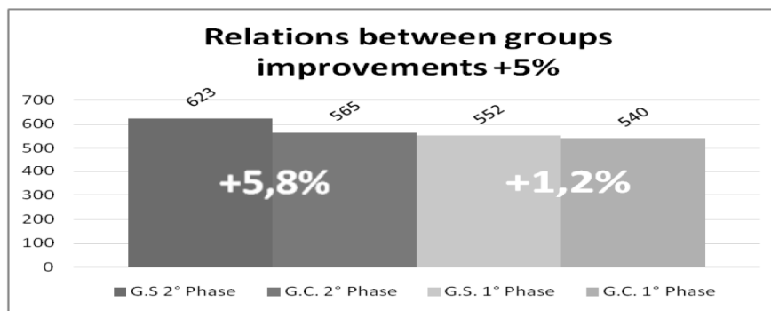
Fig. 2.2: Comparison of the difference between the two groups in input and ongoing showing an improvement of +5%
